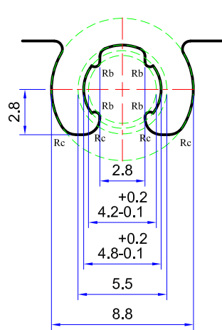
Detail 'K9' Scale 3:1
